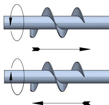
LEFT HAND SCREW FLIGHT
