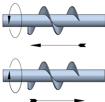
RIGHT HAND SCREW FLIGHT
